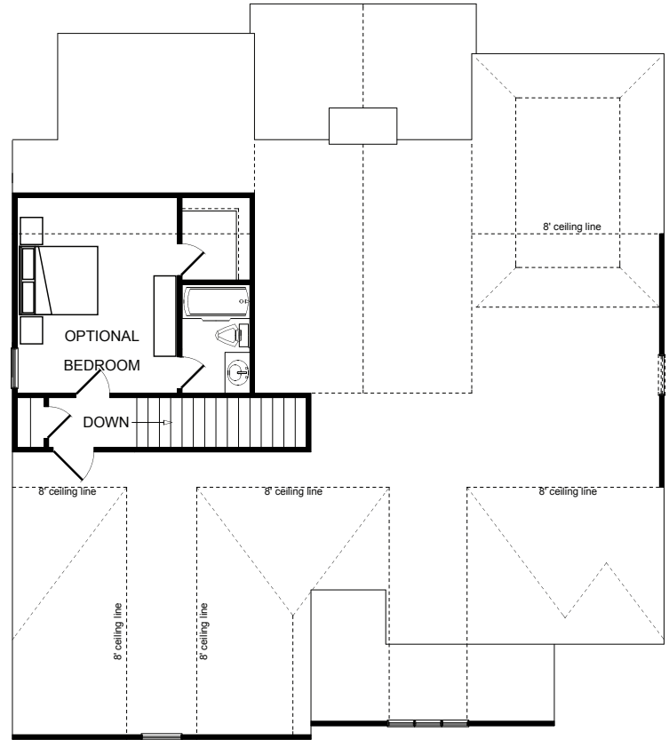
UPPER LEVEL
